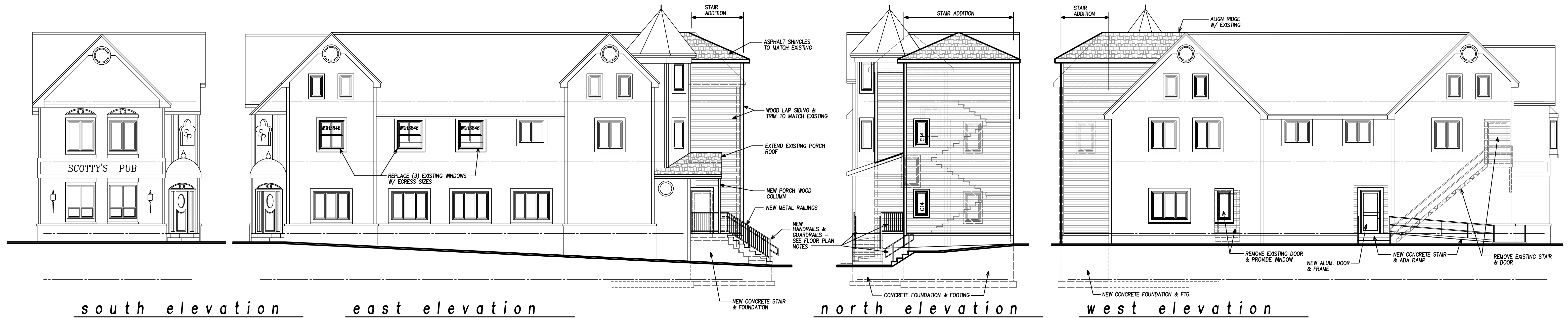
proposed elevations
