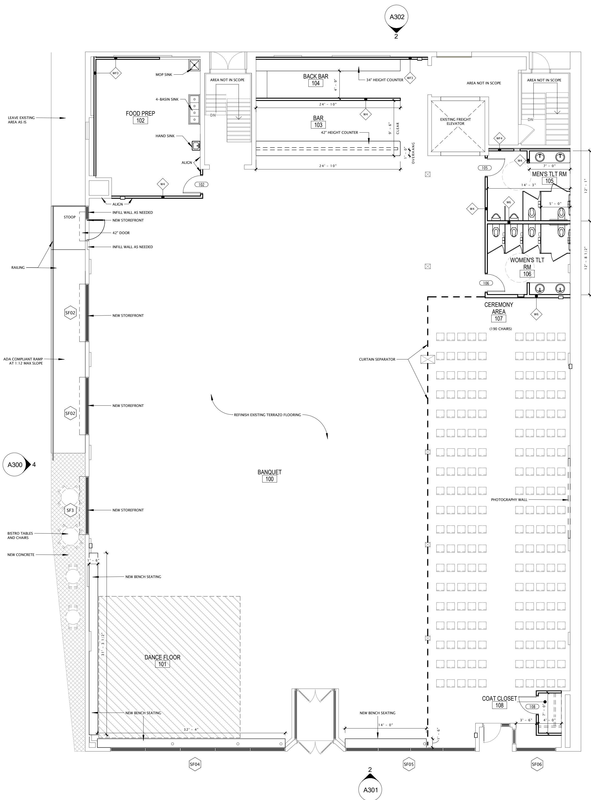
2 1ST FLOOR - PROPOSED ALTERATION
