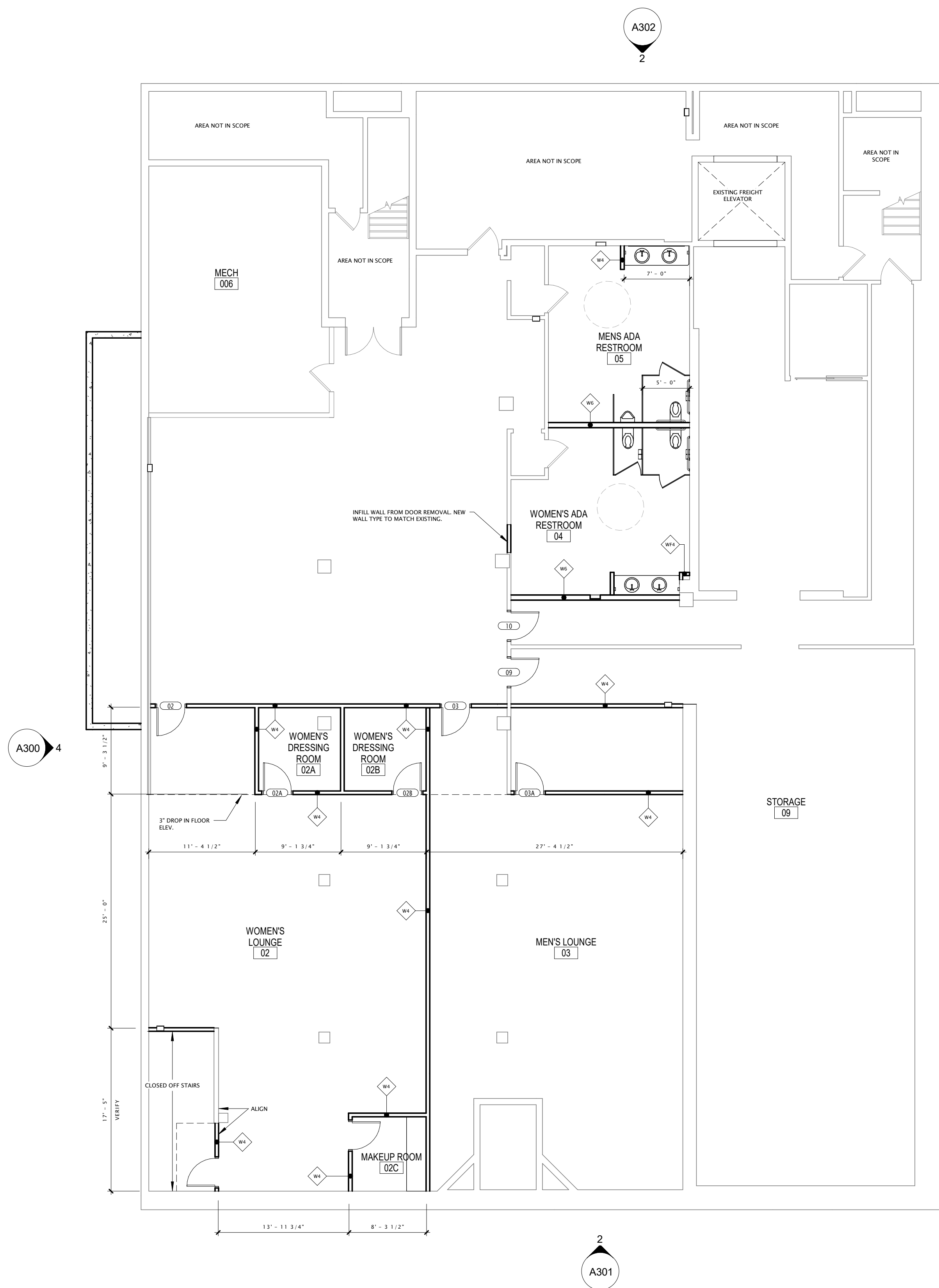
1 LOWER LEVEL - PROPOSED ALTERATION
