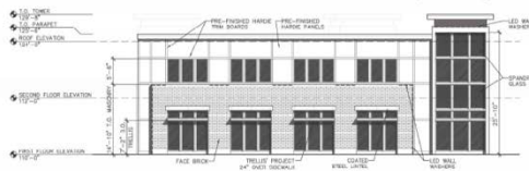
WEST ELEVATION SCALE: 1/8" = 1'-0" @ 34x22 (1/16" @ 11x17)
