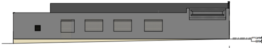
3 WEST ELEVATION - EXISTING
