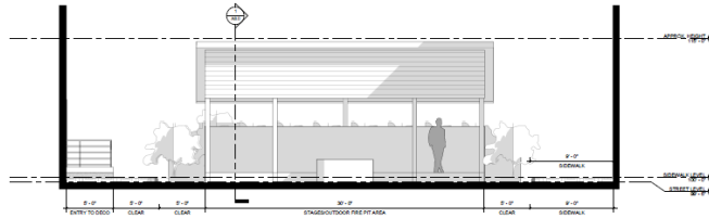
2 E-W SECTION 1/4" = 1'-0"
