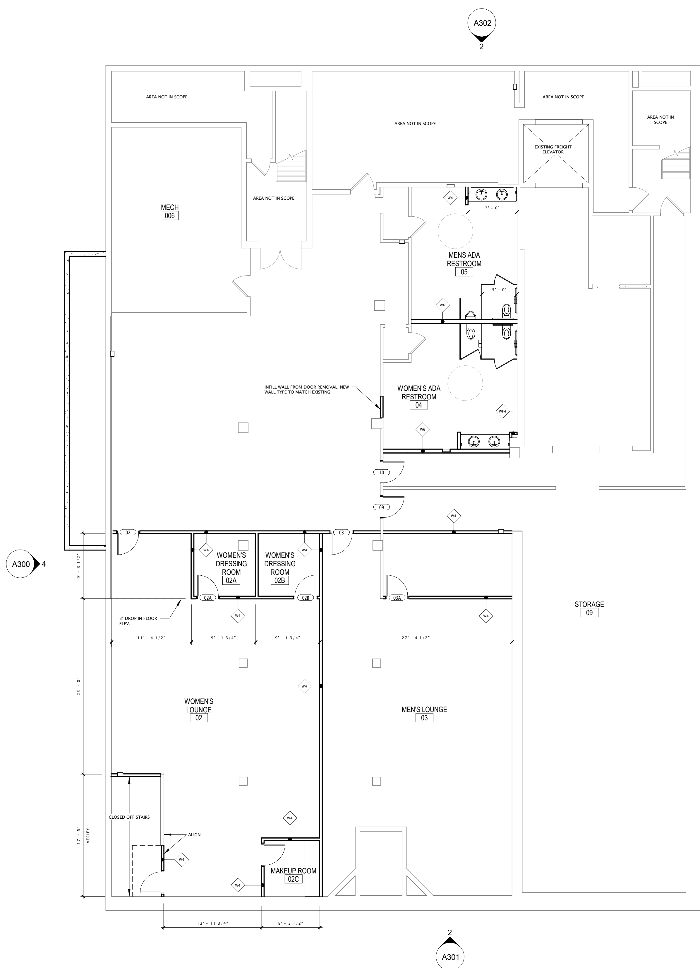
1 LOWER LEVEL - PROPOSED ALTERATION 1/8" = 1'-0"
