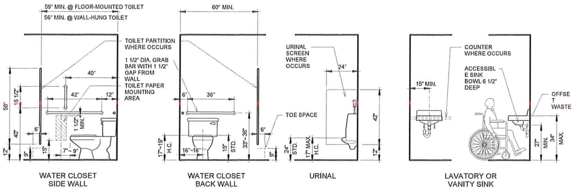
2 ADA Restrooms 3/8" = 1'-0"
